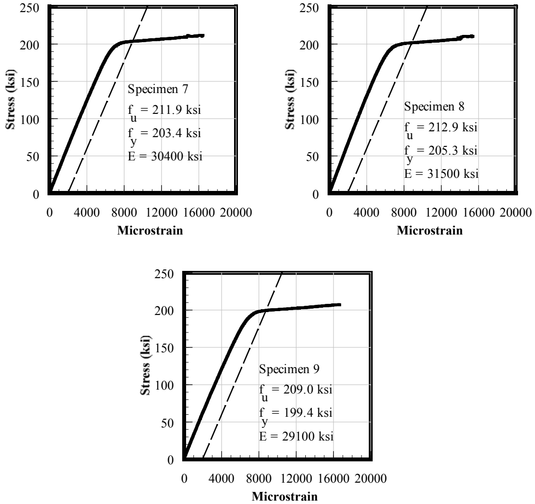
Figure 6 (cont'd) – Stress vs. Strain Results – Welded Specimens
