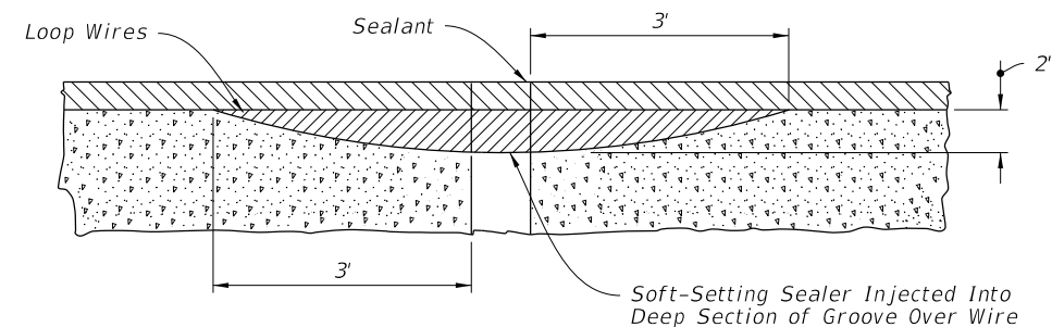
VERTICAL SECTION
