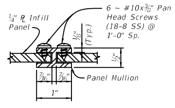
SECTION C-C PANEL/SPLICE CONNECTION
