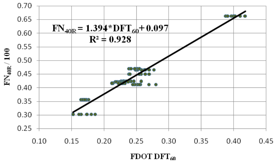
FIGURE 13 Florida DOT DFT 60 vs. Ribbed Tire Friction Number (FN 40R ).
