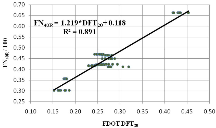
FIGURE 11 Florida DOT DFT 20 vs. Ribbed Tire Friction Number (FN 40R ).
