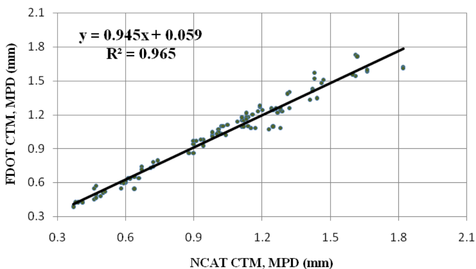
FIGURE 7 Florida DOT CTM vs. NCAT CTM Data, MPD (mm).
