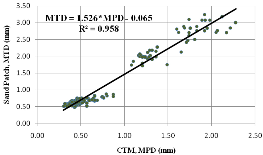
FIGURE 22 Correlation of MTD with MPD on Florida Pavements.
