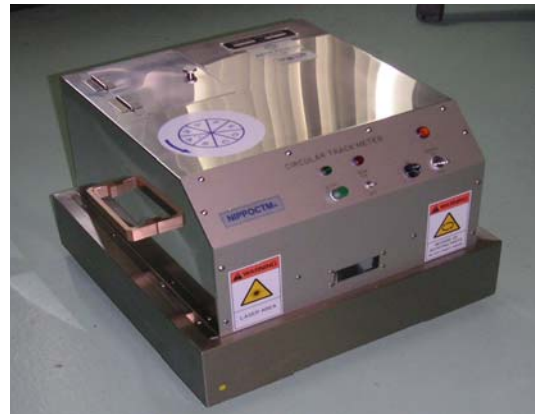
b) Circular Track Meter (CTM).
