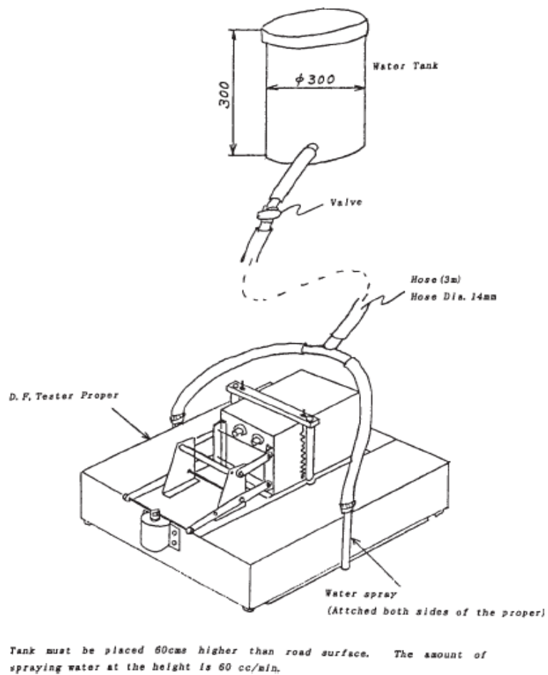
Figure A 5 The DFT Water Supply Tank [39]
