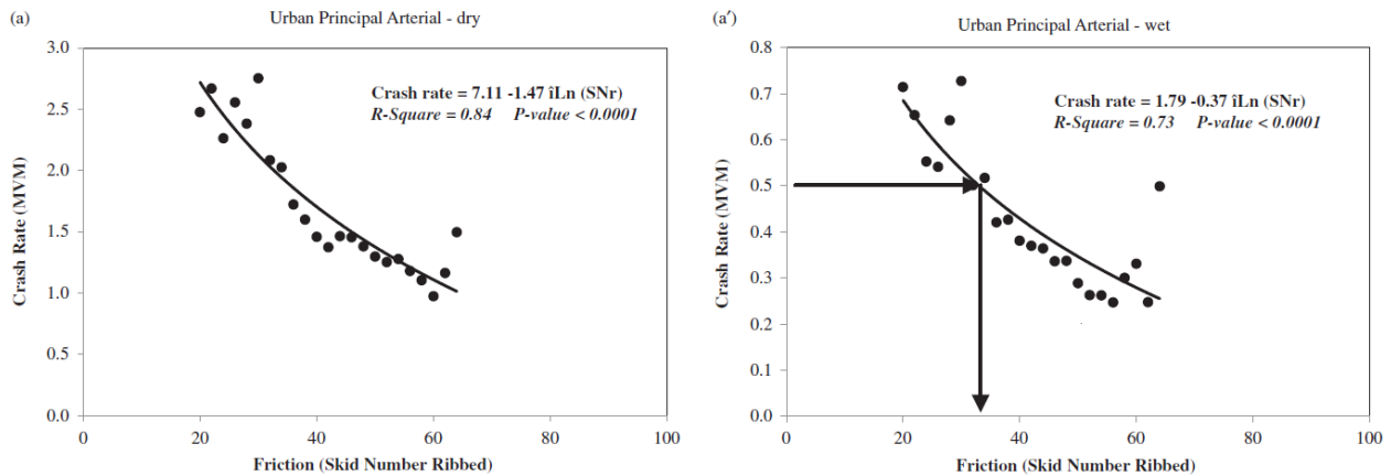
Figure 10: Example of Crash Rate versus Friction from New Jersey (Najafi et al. 2017)
