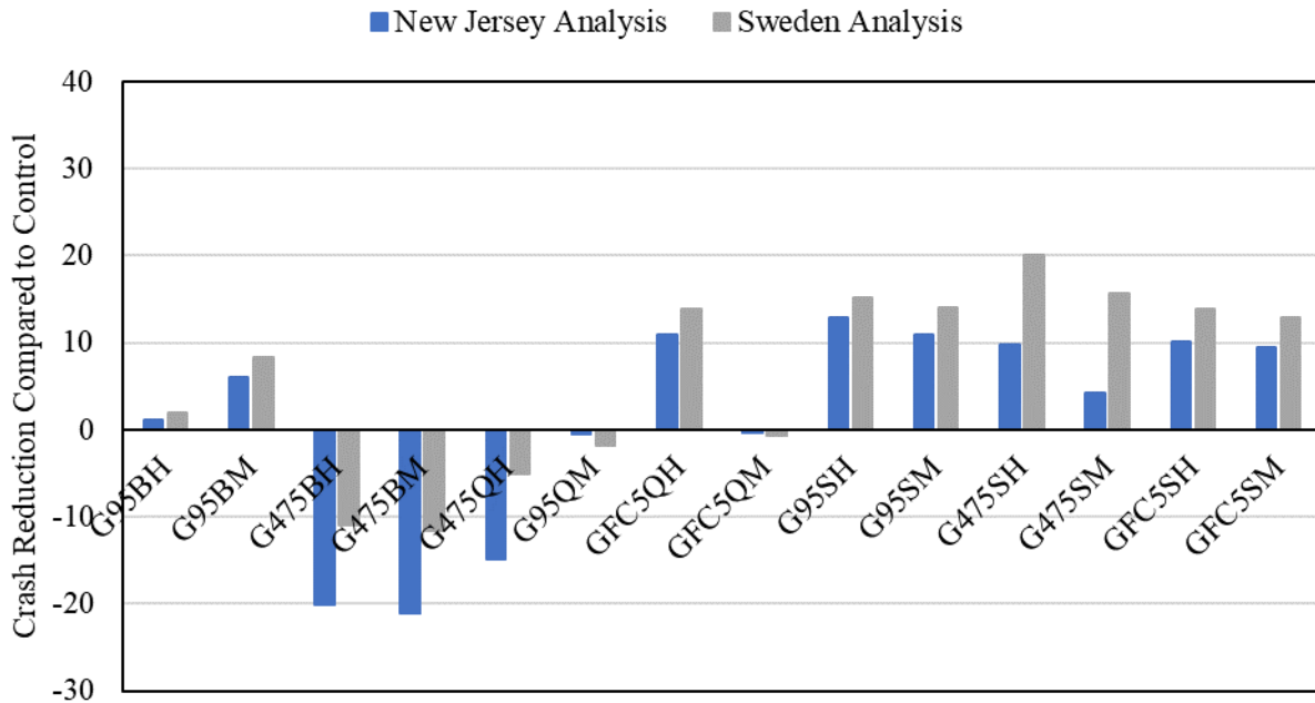
Figure 50: Crash Reduction Potential Compared to Control – Granite
