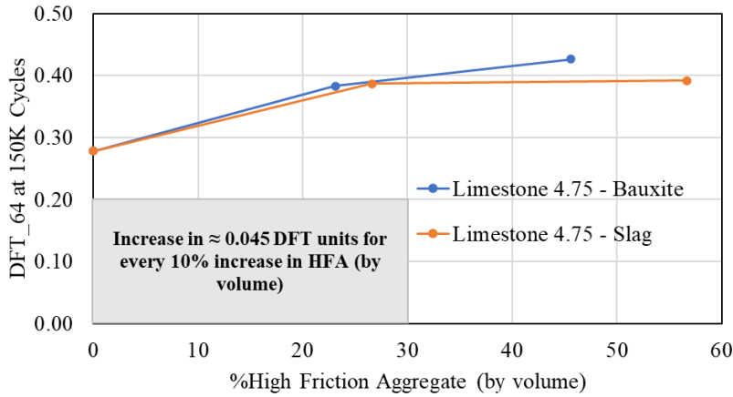
Figure 30: DFT_64 versus %HFA (Limestone FC-4.75 Only)
