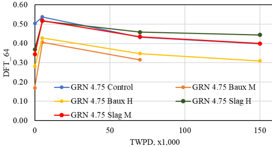
Figure 24: DFT Results – GRN FC-4.75 Mixes
