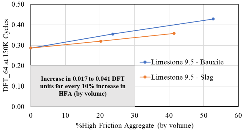
Figure 31: DFT_64 versus %HFA (Limestone FC-9.5 Only)
