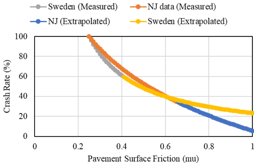
Figure 44: Estimated Crash Rate Response to Pavement Friction
