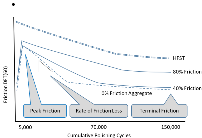
Figure 12: Concept of Percent Friction Aggregate Influence on Friction Performance
