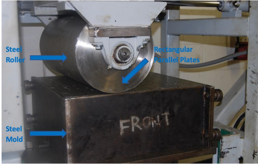
Figure 15. NCAT Linear Kneading Compactor (NCAT, 2016)
