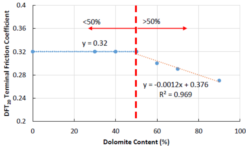
Figure 3: Relationship between Terminal DFT and Dolomite Content (West, et al. 2021)
