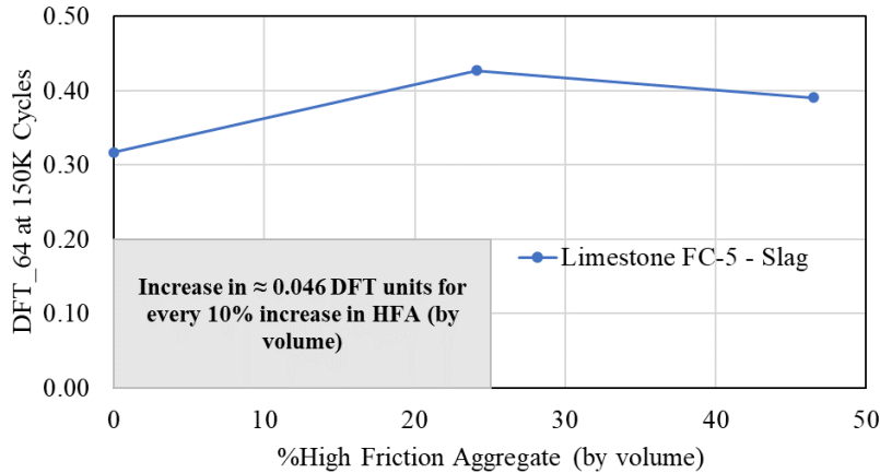
Figure 32: DFT_64 versus %HFA (Limestone FC-5 Only)
