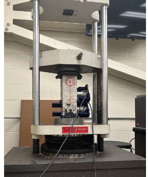
Testing setup for small-scale 50-kHz and 500-kHz testing on block specimens.
