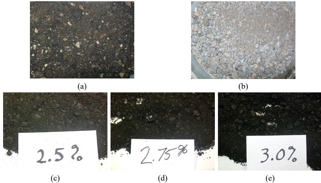
Figure 1. Georgia RAP Samples: (a) Heated RAP, (b) Post-ignition RAP Aggregate, (c, d, e) Post-ignition RAP Aggregate Mixed with Different Amounts of Virgin Binder (Hines, 2012)
