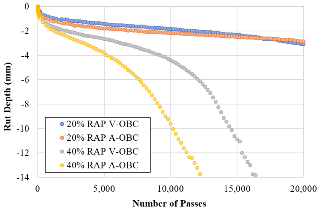
Figure 26. HWTT Rutting Curves of GRN Mixtures at V-OBC and A-OBC
