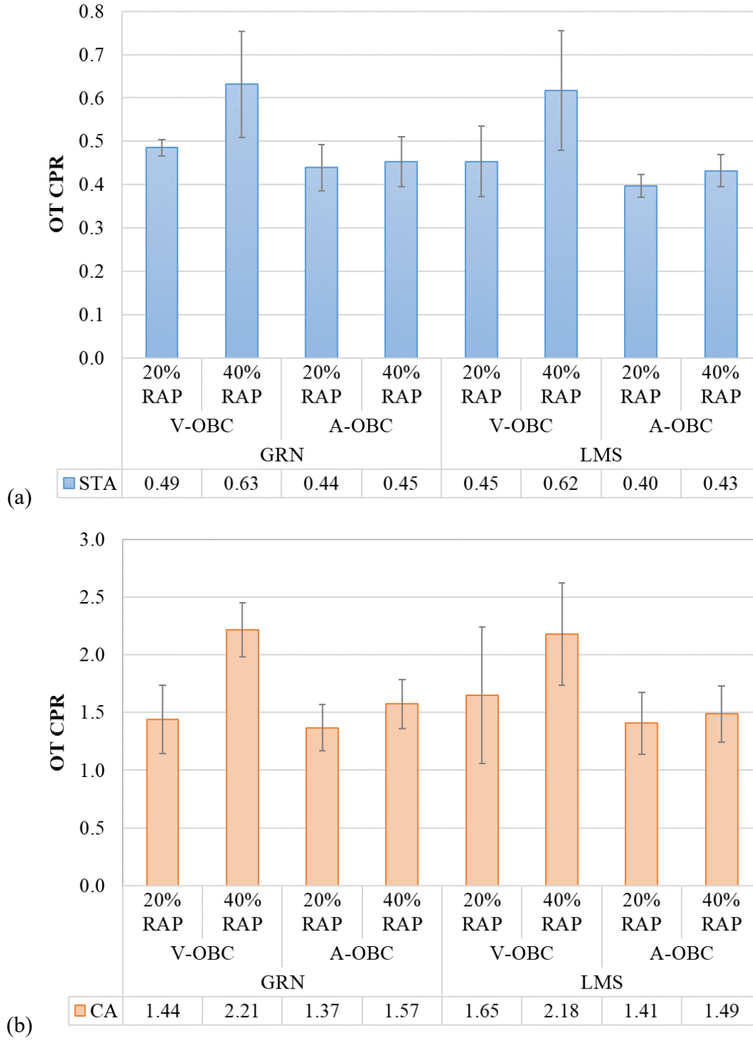
Figure 19. OT CPR Results: (a) STA Condition, (b) CA Condition
