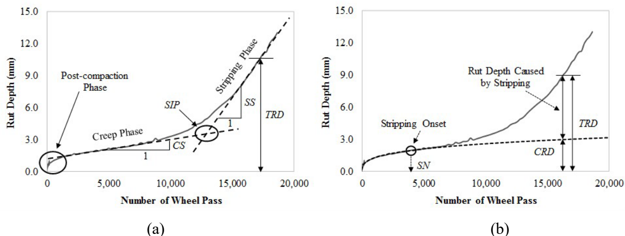
Figure 25. HWTT Results: (a) Typical Three-phase Rutting Curve, (b) Illustration of CRD versus TRD (Yin et al., 2020)
