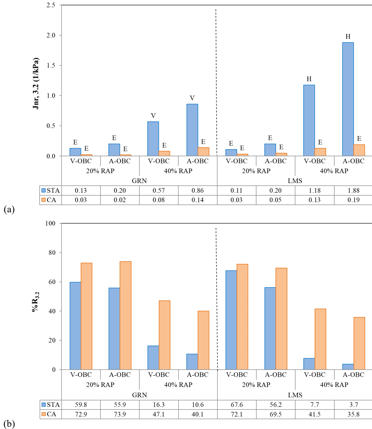
Figure 38. MSCR Results: (a) J_{nr,3.2} , (b) \%R_{3.2} . Where H = heavy traffic loading (10-30 million ESALs or 20-70 km/h), V = very heavy traffic loading (>30 million ESALs or <20 km/h), E = extreme traffic loading (>30 million ESALs and <20 km/h).
