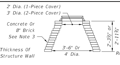
BRICK OR CONCRETE PRECAST CONCENTRIC CONE TYPE 8 MANHOLE TOPS
