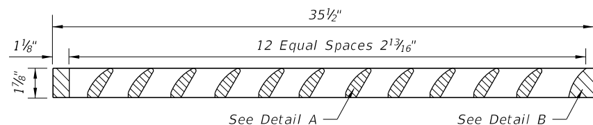
SECTION
