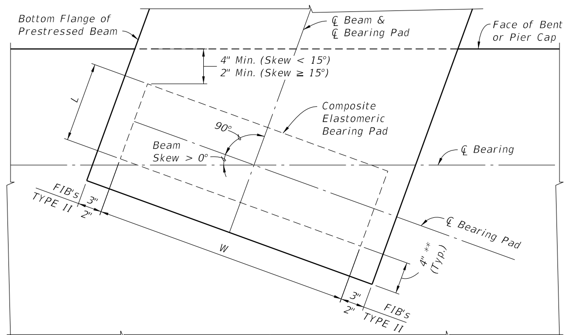
PARTIAL PLAN WITH SQUARED END BEAM (Use Index 20512) (Beam Skew > 0°; Bearing Skew = 0°)
