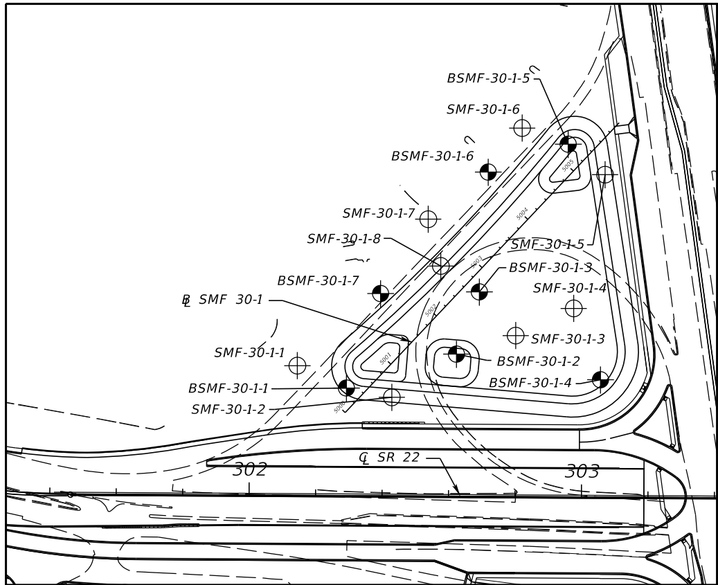
BORING LOCATION
