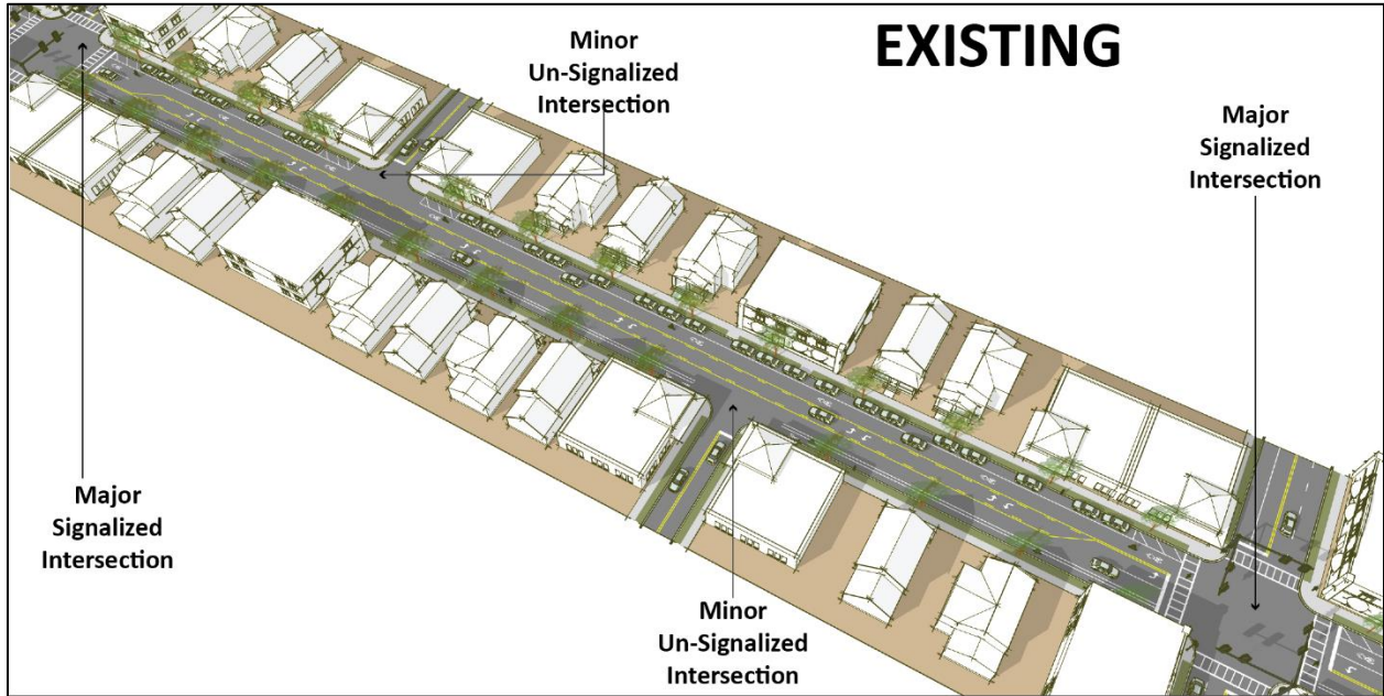
Figure 202.3.2 Concept Sketch – Mark Crossings to Emphasize Short Blocks
