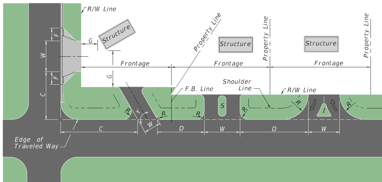
Figure 214.1.1 Driveway Terminology
