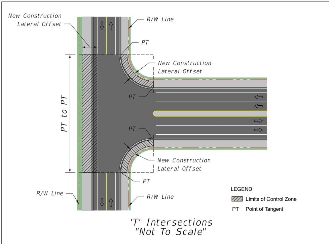
Figure 215.2.5 'T' Intersection
