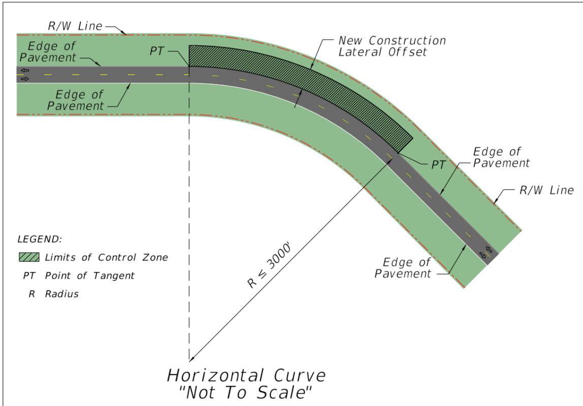
Figure 215.2.12 Horizontal Curve
