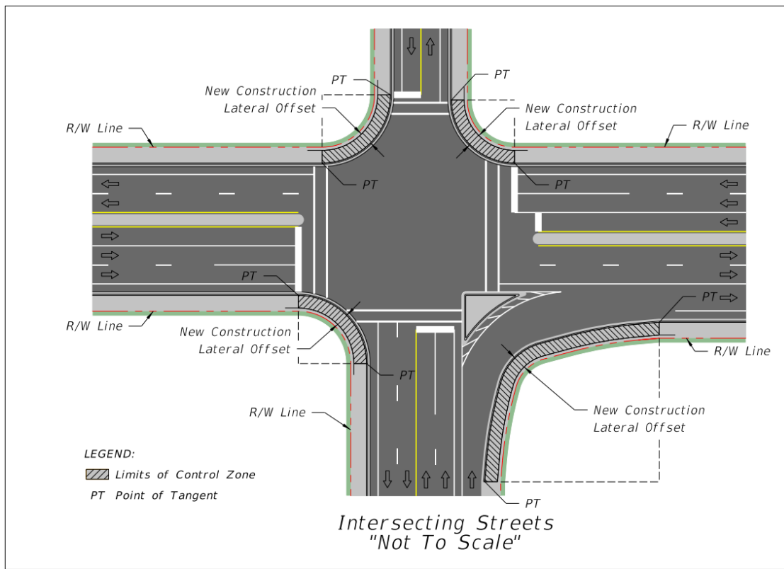
Figure 215.2.4 Intersection Radii
