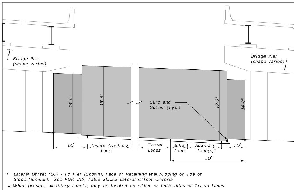
Figure 260.6.4 Curbed Roadway ≤ 45 mph – Section through Bridge
