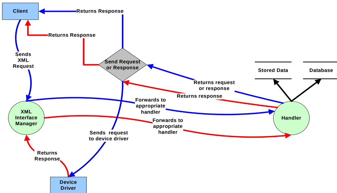
Figure 2-6 - XML Handling
