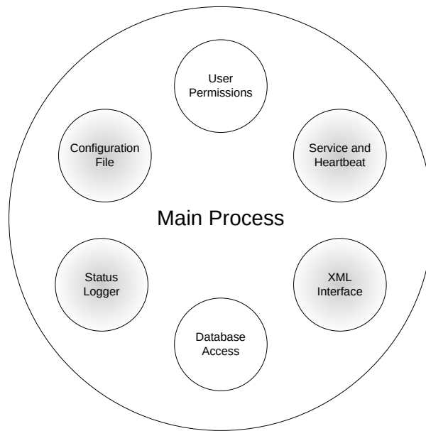
Figure 2-1 - Generic Capabilities
