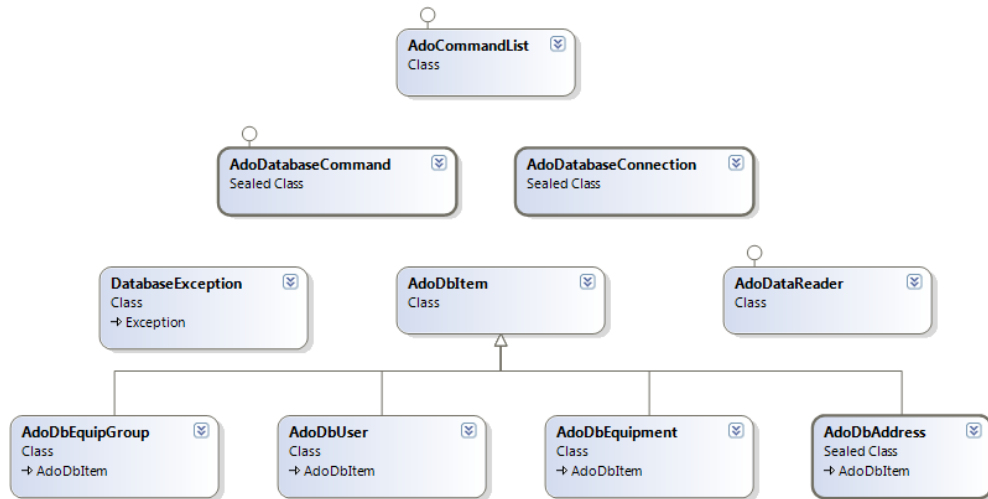
Figure 2-8 - Database Classes
