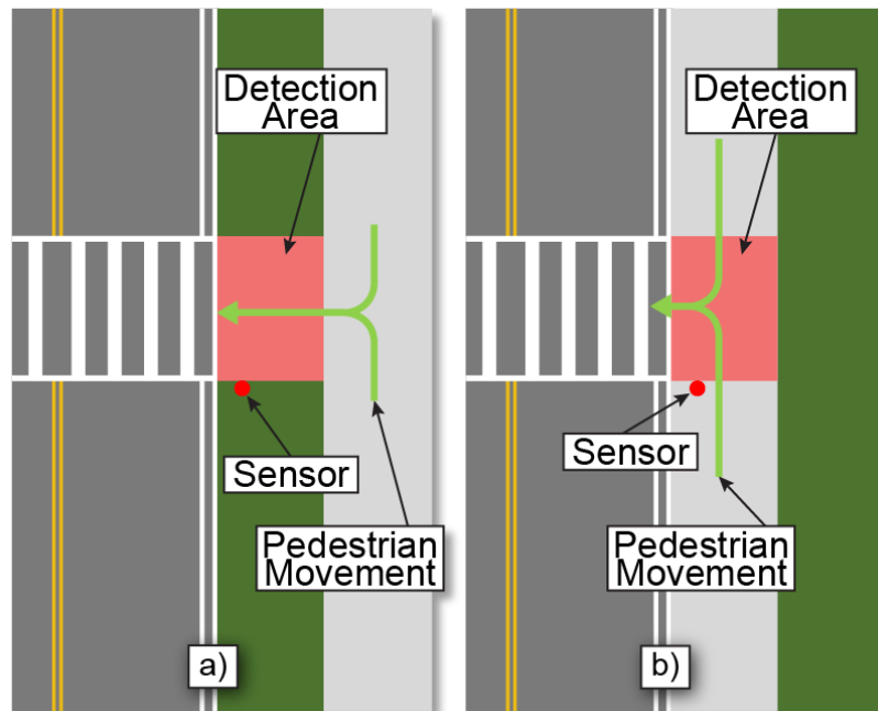
Figure 5.2-12. Sidewalk Location Options for Passive Pedestrian Detection
