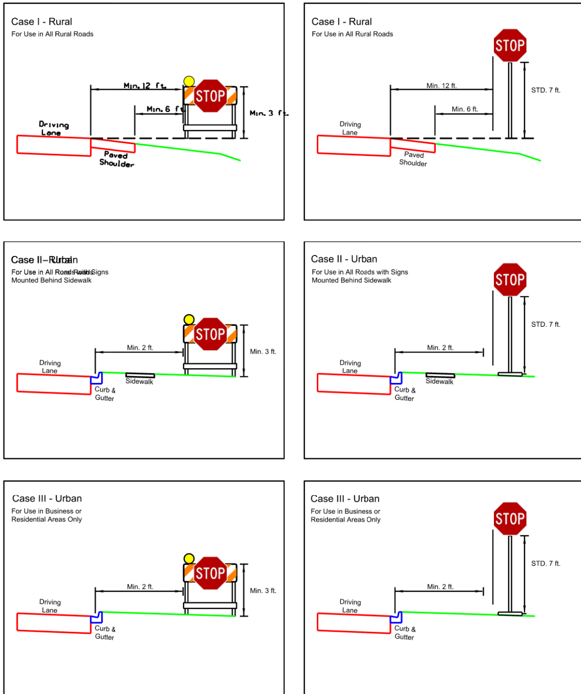
Figure 2.38-6. Temporary Signaling for Power Outage – Sign Dimensions
