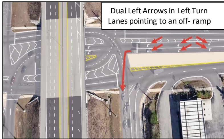
Figure 4.2-6. Dual Left Turn Lanes with Left Turn Arrows
