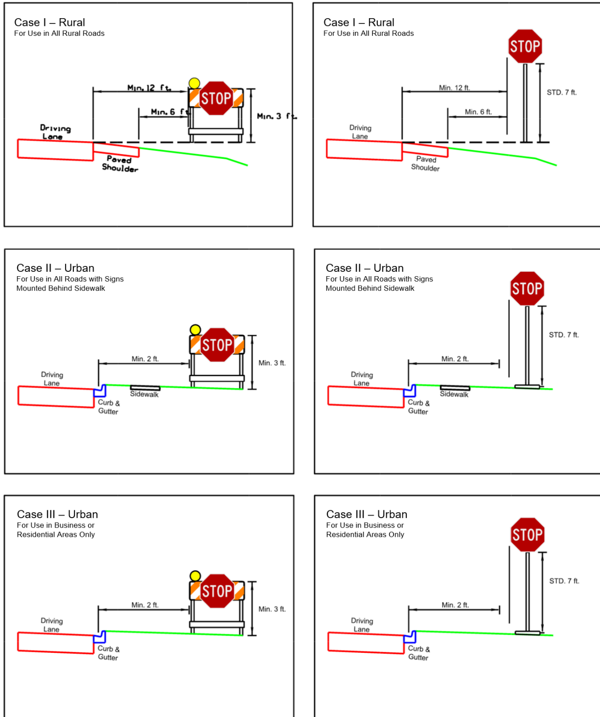
Figure 2.38-6. Temporary Signage for Power Outage—Sign Dimensions
