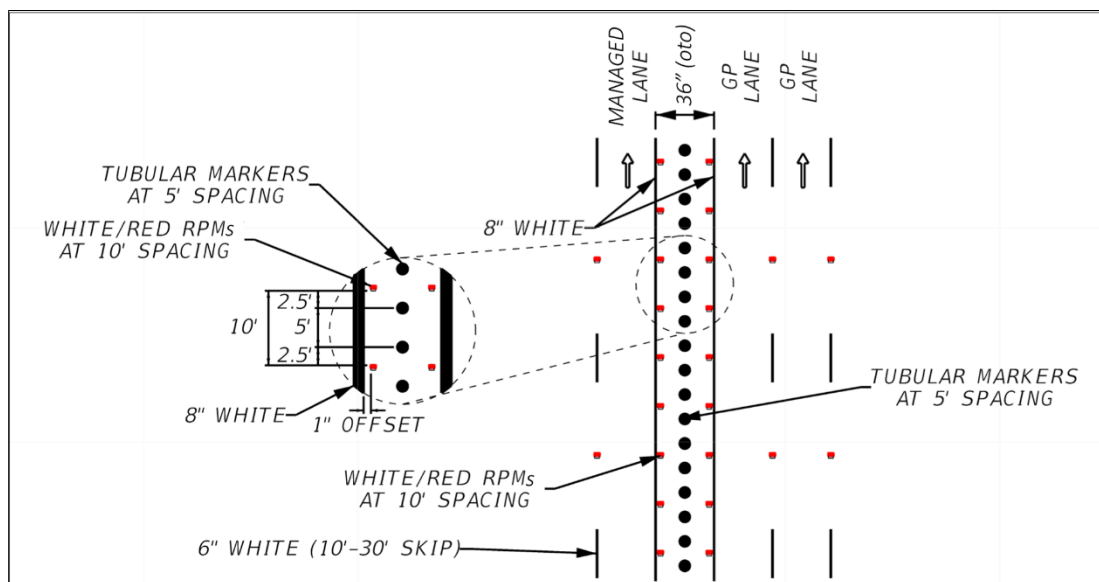
Figure 4.5-1. Separation Detail
